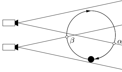
Fig. 1. Simulation setup. The object moves on a circular path. At points \alpha and \beta , object loss may occur due to limited zoom motor speed.
