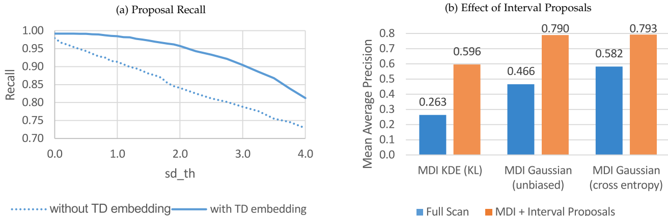
Figure 11. (a) Recall of interval proposals without time-delay embedding and with \kappa = 6, \tau = 2 on the synthetic data set for different proposal thresholds. (b) Effect of interval proposals on the Mean Average Precision of different variants of the MDI algorithm on the synthetic data set.
